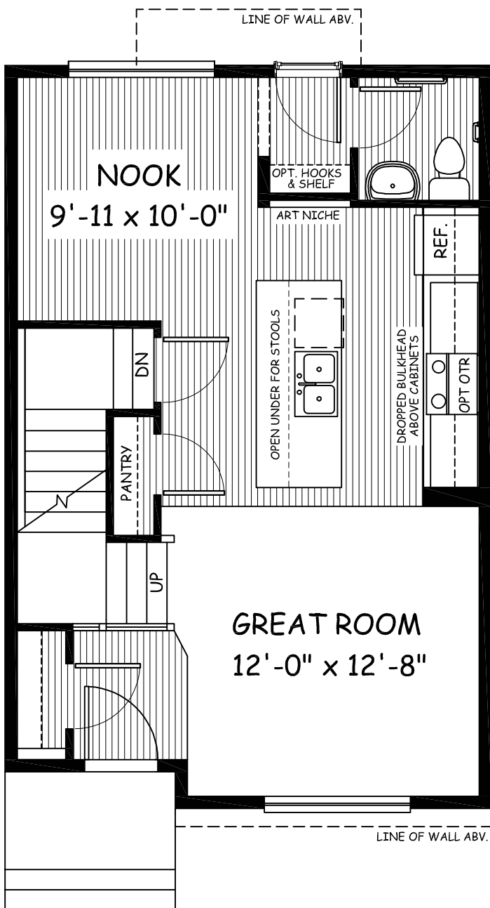
Main Floor 600 sqft
